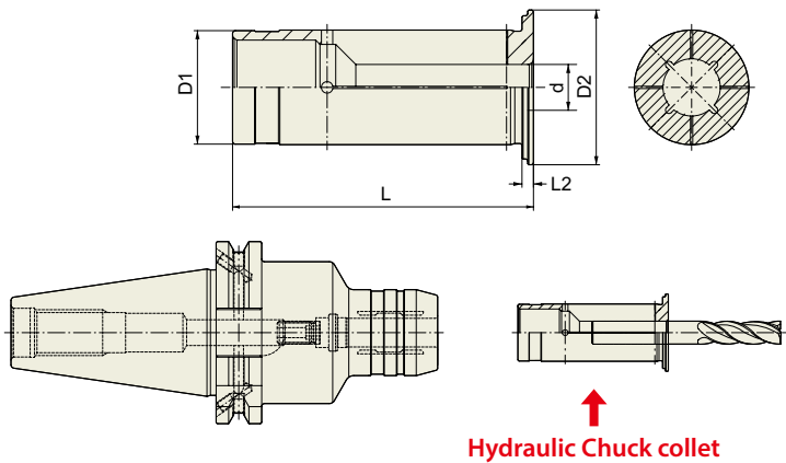
Hydraulic Chuck collet
